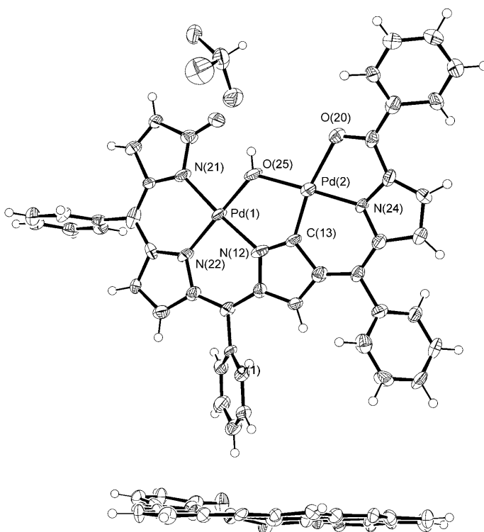
Figure 2. An ORTEP plot of the crystal structure of dipalladium complex 7 ·CHCl 3 (thermal ellipsoids are drawn at the 30% probability level). Bottom: side view of the molecule (CHCl 3 and phenyl substituents omitted).
