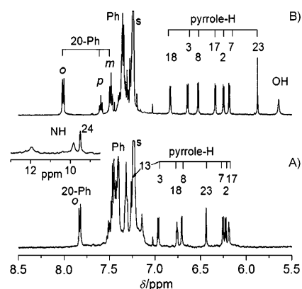
Figure 1. 1 H NMR spectra (500 MHz, CDCl 3 , 300 K) of 5 (A) and palladium complex 7 (B). Assignments: pyrrole-H=pyrrole resonances; 20-Ph=signals of phenyl substituent on C(20); Ph=remaining phenyl signals; s=residual solvent peak. Inset in A shows the NH peaks of 5 .
