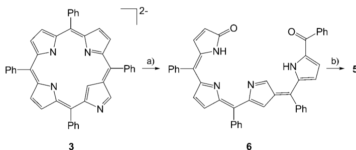
Scheme 2. Photooxidation of the N-confused tetraphenylporphyrin dianion. a) O 2 , h \nu ; b) MeOH.
