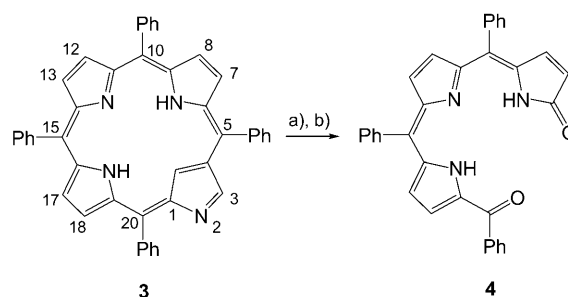
Scheme 1. Degradation of the N-confused tetraphenylporphyrin. a) Cu(OAc) 2 , O 2 , toluene; b) H + .
