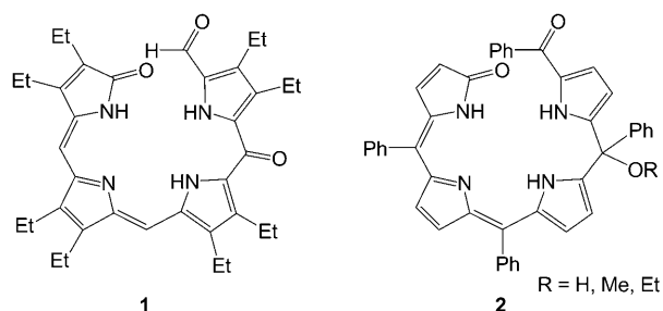
Scheme 1. Degradation of the N-confused tetraphenylporphyrin. a) Cu(OAc) 2 , O 2 , toluene; b) H + .
